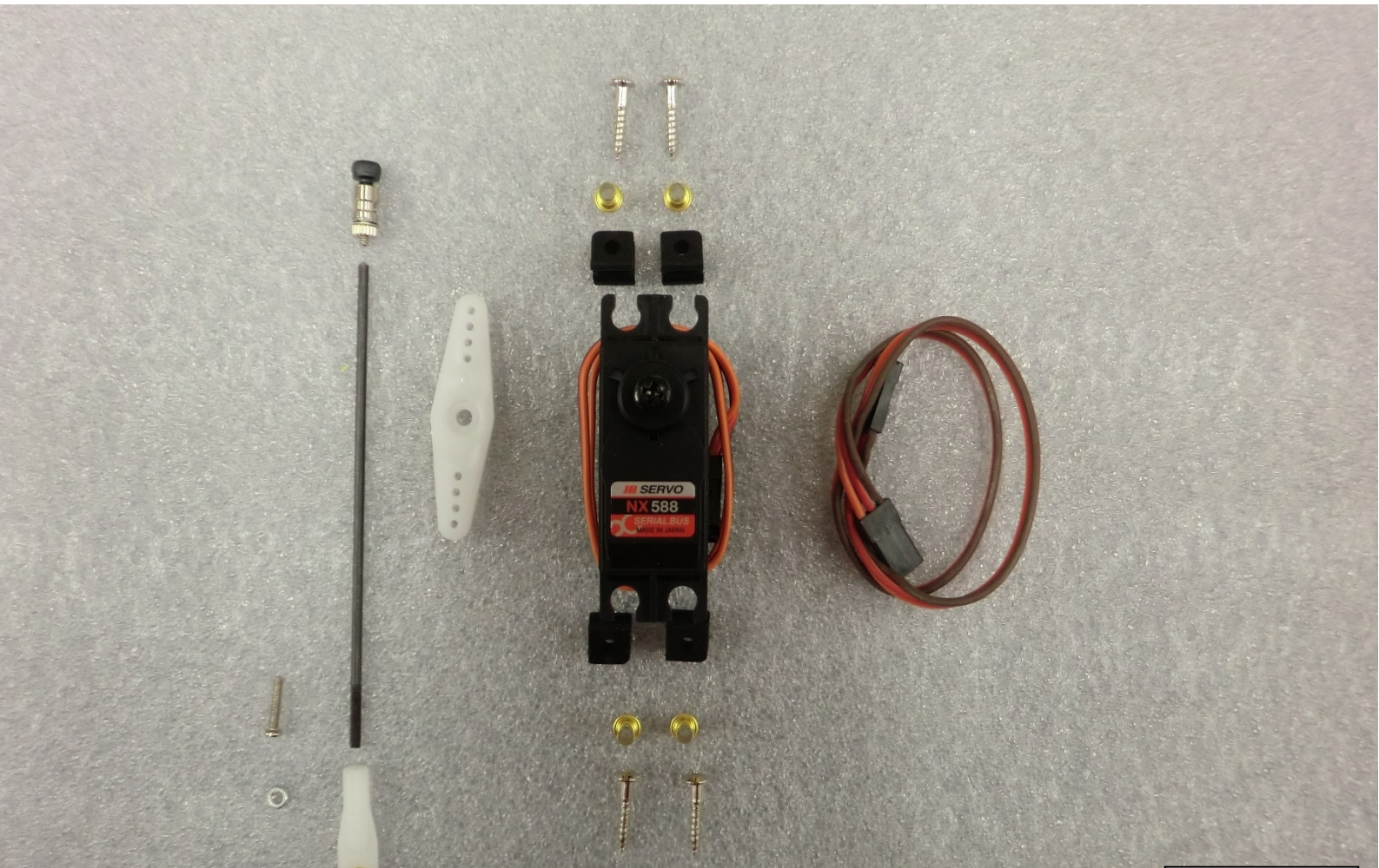
AILERON SERVO
