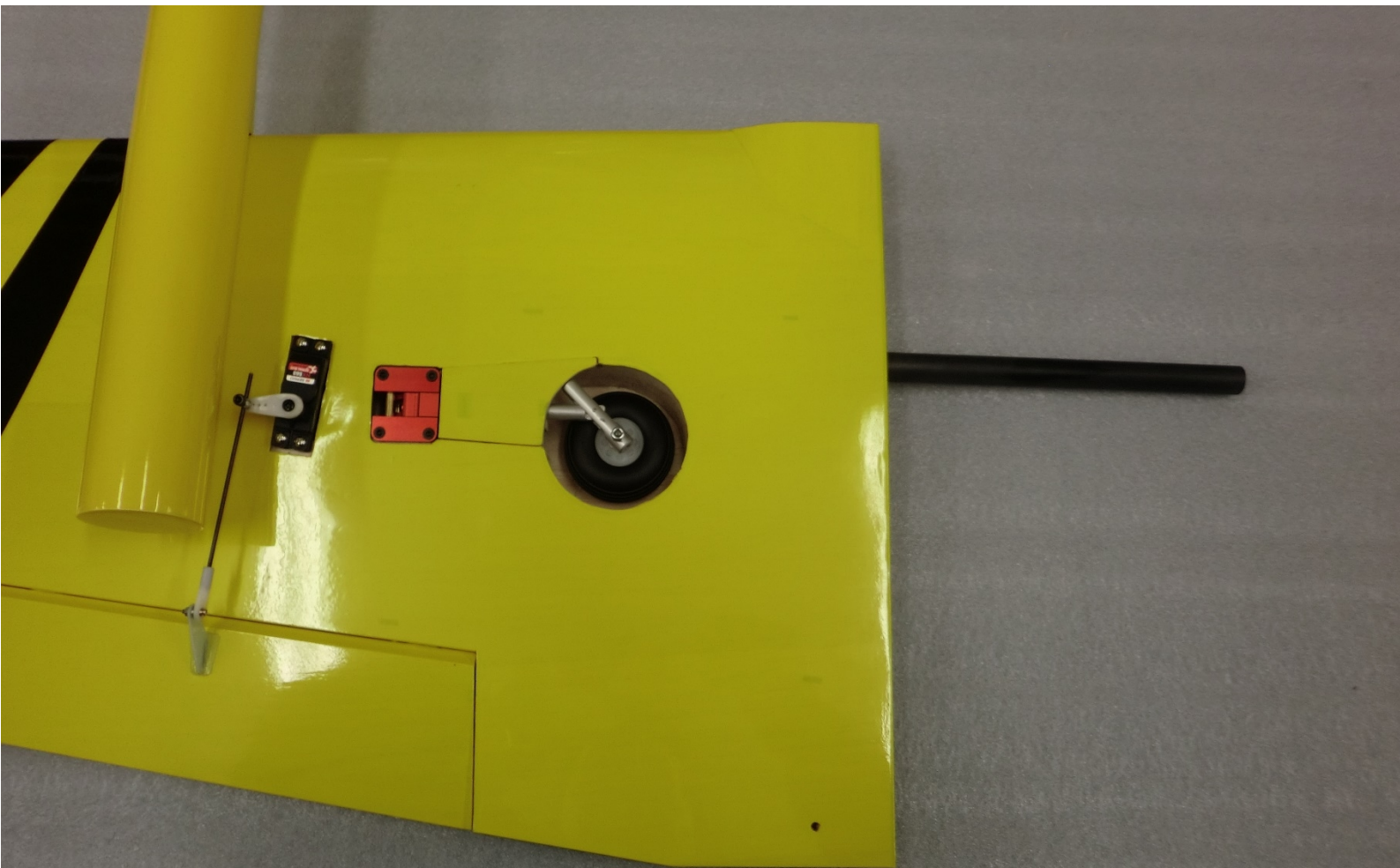
FIXING WINGS
