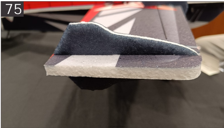
75. If desired, locate these smaller side force generators that will be glued into the counterbalances of the ailerons.
