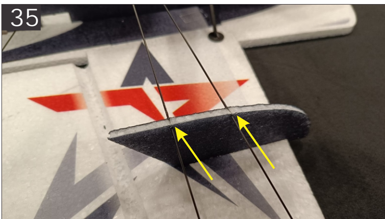
35. Here is how the carbon rods went through the slots in wing truss supports, slid in about 1mm down into these slots and glue it together.
