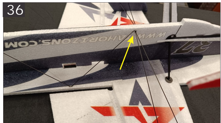
36. Shown above is how the wing bracing rods are glued just behind the undercarriage to the fuselage wall.
