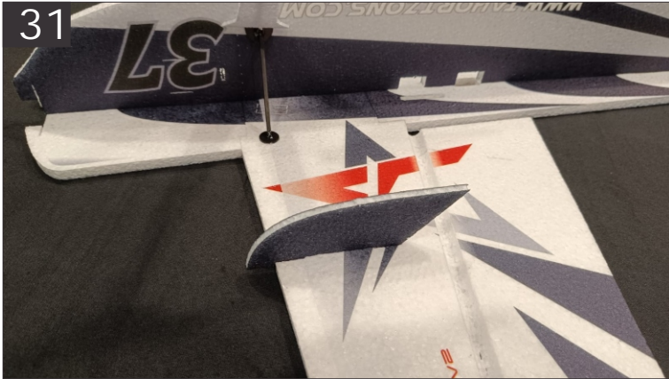
31. Locate and glue the half part of SFG works as wing truss support, glue it in pre-cut slot like shown in the picture.
