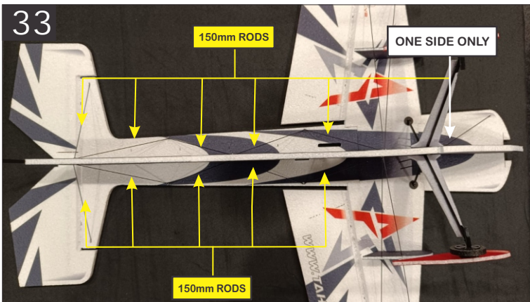
33. Carbon rod needs to sit couple of mm into the foam before gluing, Just put a small drop of HV Cyno to glue it. (Please Refer to above image for the reference)
