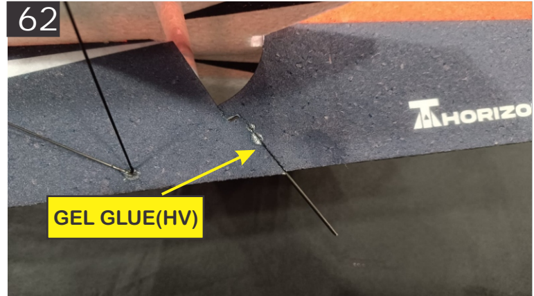
62. Now with the top portion installed glue the rear part to the flat carbon rod that we glued earlier.
