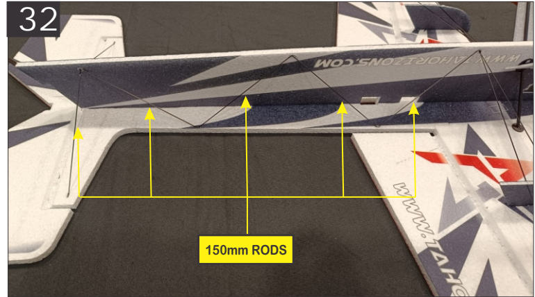
32. Rods bracing the fuselage are 1mm dia 150mm L. Please refer to the above image for reference.
