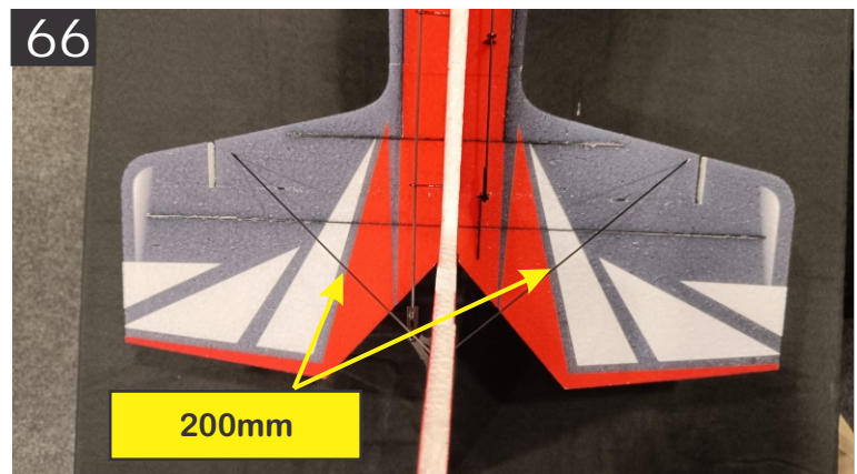
66. Shown above are the 200mm X 2 carbon rod that will go on each side of the fuselage. It will be used to strengthen the horizontal stab and vertical stab.
