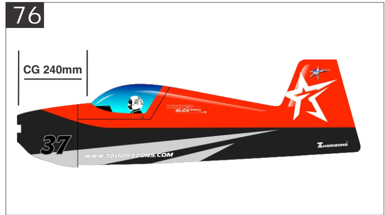
76. Initial CG is located 240mm from the nose of the aircraft (Not from the motor)
