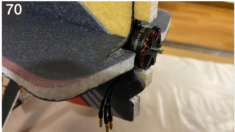
70. Enlarge the pre cut holes over the mount according to need and install the motor on it.
